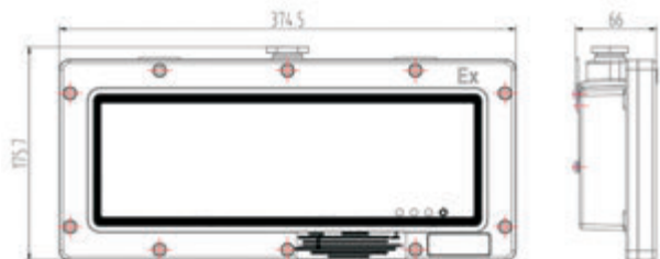
Drawing of dimension (Dimensions in mm)
