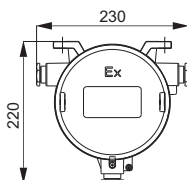
Explosion proof ballast box
