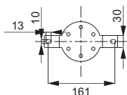
Ceiling mounting (standard)
