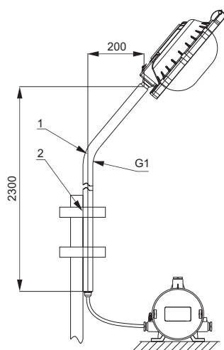
Guardrail mounting
