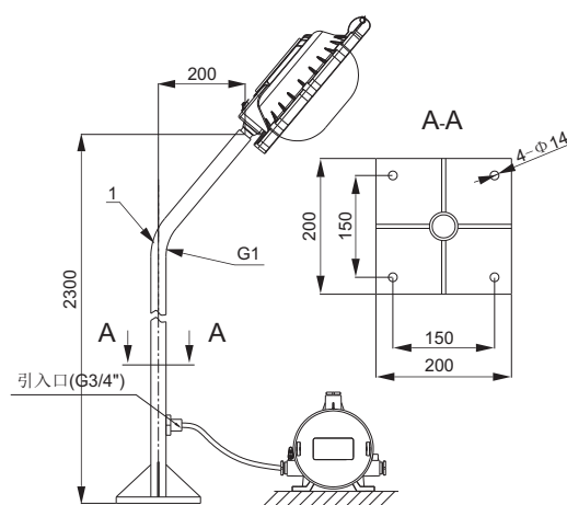
Flange mounting
