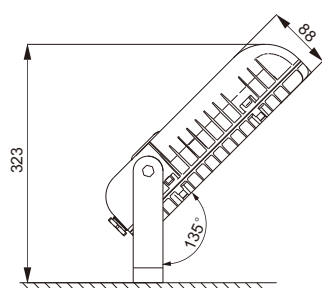
Seat mounting
