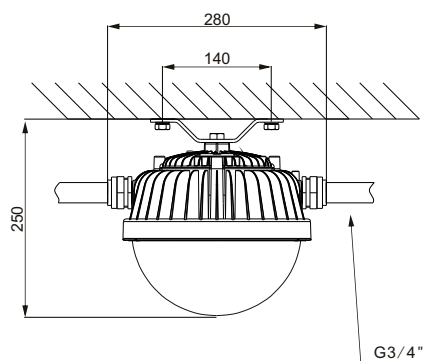
Ceiling mounting
