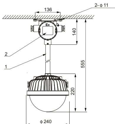
Pole mounting
