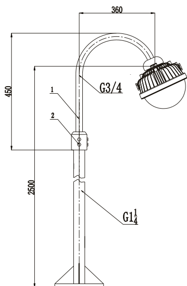
Flange mounting
