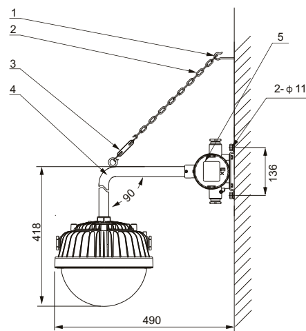
Wall mounting 90°
