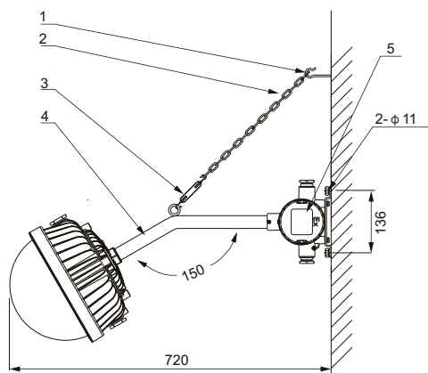
Wall mounting 150°
