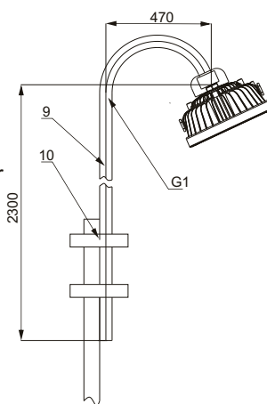
Fence Mounting
