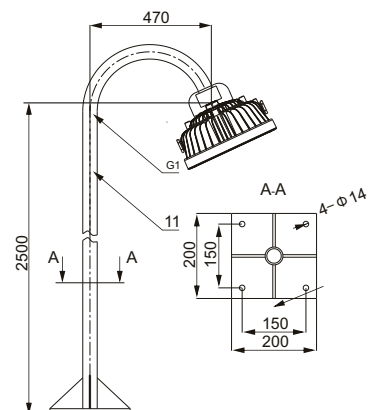
Flanged Mounting
