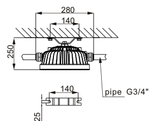
Ceiling mounting
