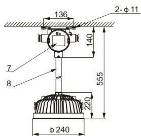
Pole mounting
