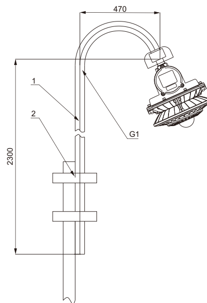
Guardrail mounting
