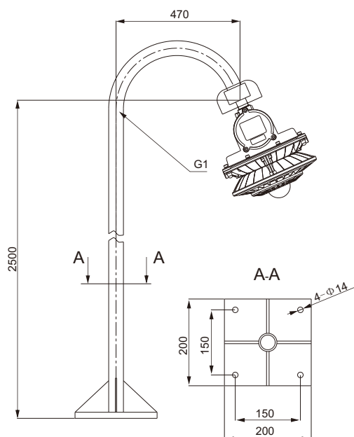
Flange mounting
