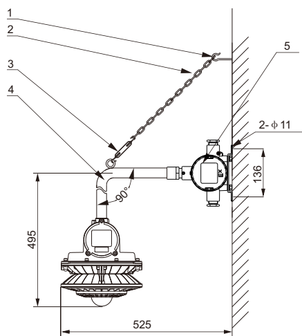
Wall mounting 90°
