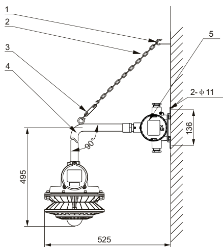
Wall mounting 90deg
