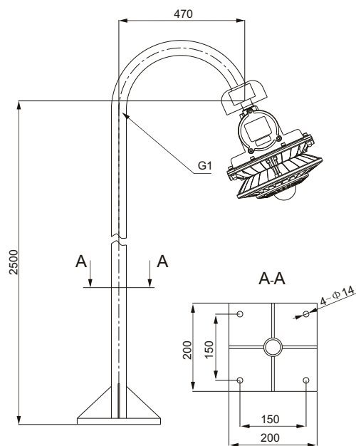
Accessories order information(Flange mounting)
