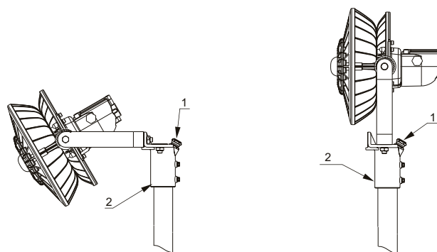
Pole mounting
