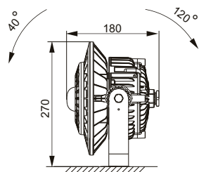
Seat mounting
