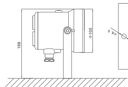
Seat installation
