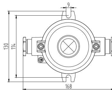
BZA5200-D Indicator light
