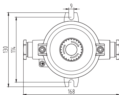
BZA5200-A1 Emergency stop button
