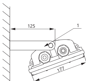
Side wall mounting (optional)
