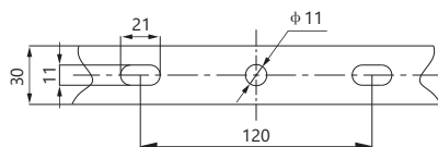
Installation dimension
