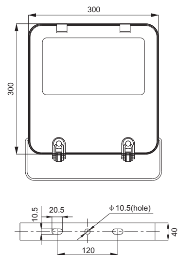
Installation Dimension
