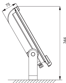
Seat mounting
