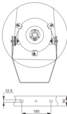
Installation Dimension
