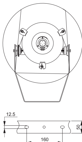
Installation Dimension
