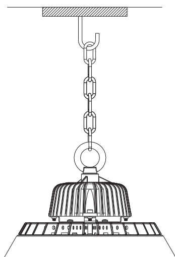
Hanging chain installation
