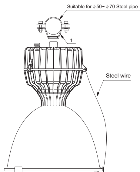
Hold hoop mounting (optional)
