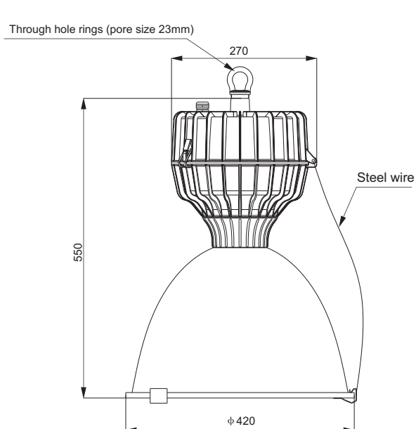
Hanging mounting (Standard)
