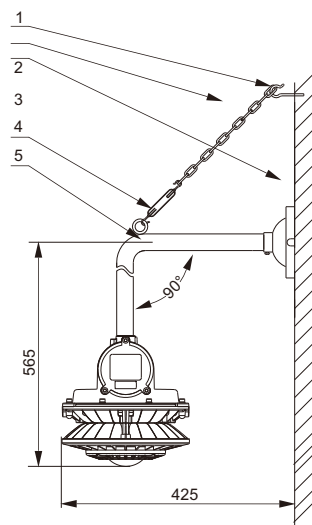
Accessories order information(Wall mounting 90°)
