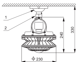
Ceiling mounting
