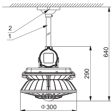
Pole mounting
