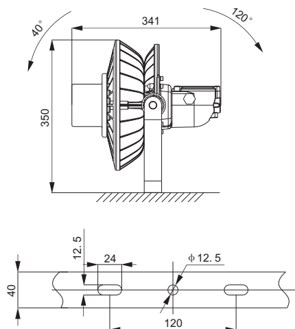
Seat mounting
