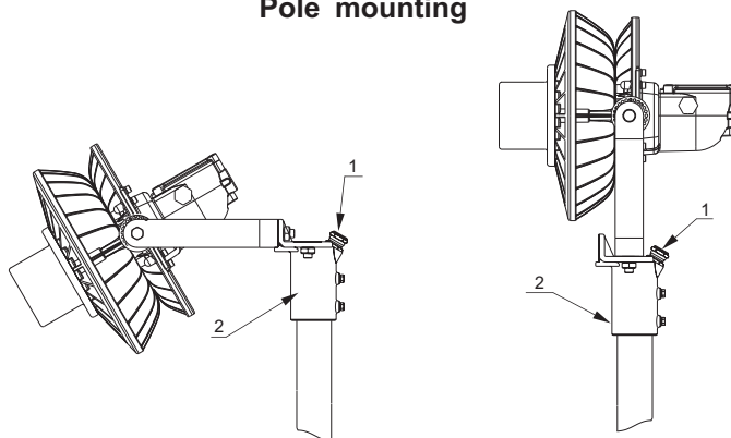
Pole mounting
