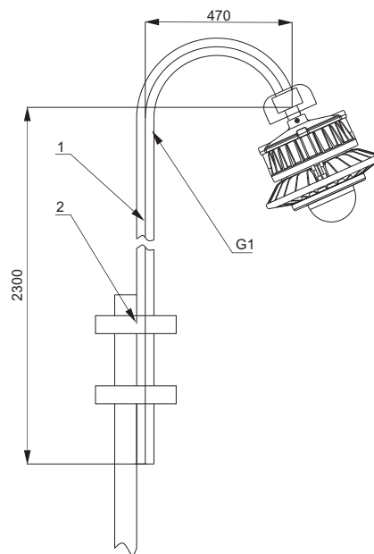
Accessories order information(Guardrail mounting)
