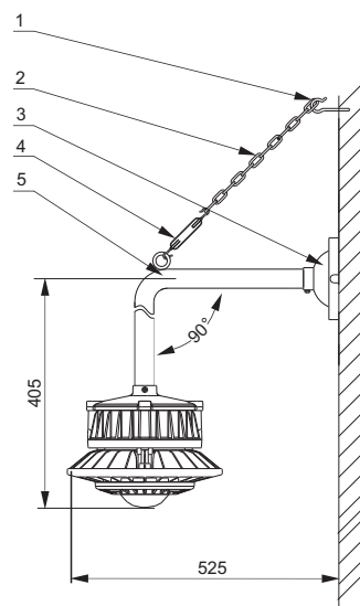
Accessories order information(Wall mounting 90deg)
