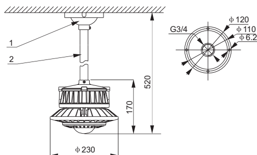
Accessories order information(Pole mounting)
